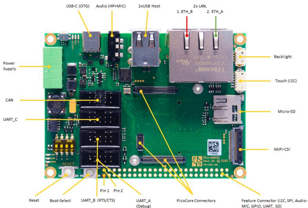
Figure 1: Top side of PicoCoreMX8MP Starterkit baseboard (PicoCoreBBDSDI – Rev. 1.30)
