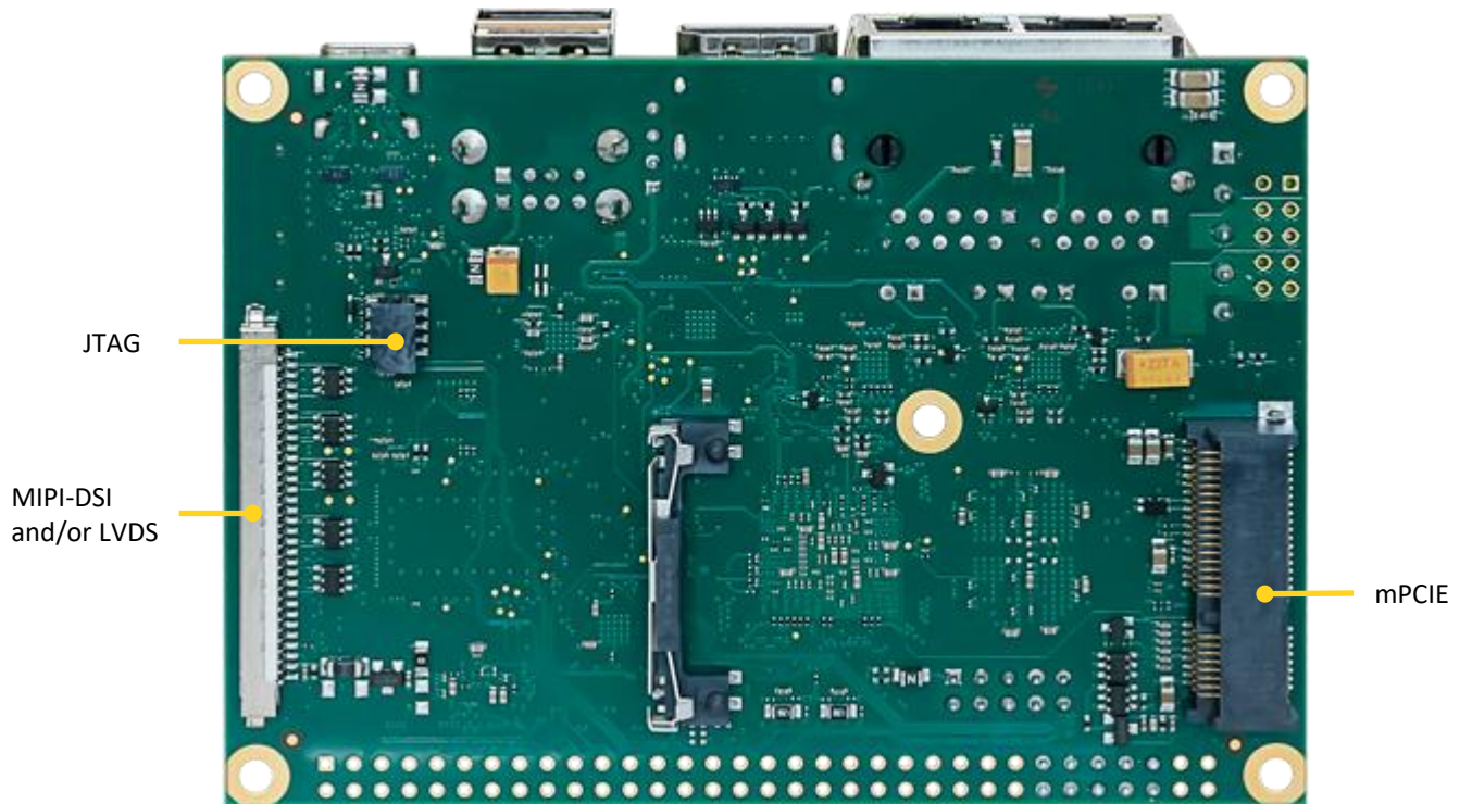
Figure 5: armStoneMX8MP-V4I bottom view
