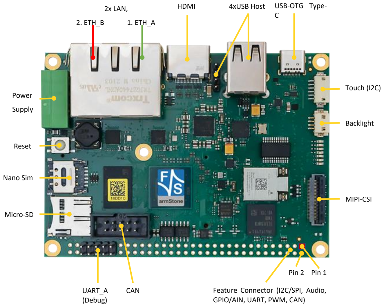
Figure 4: armStoneMX8MP-V4I top view
