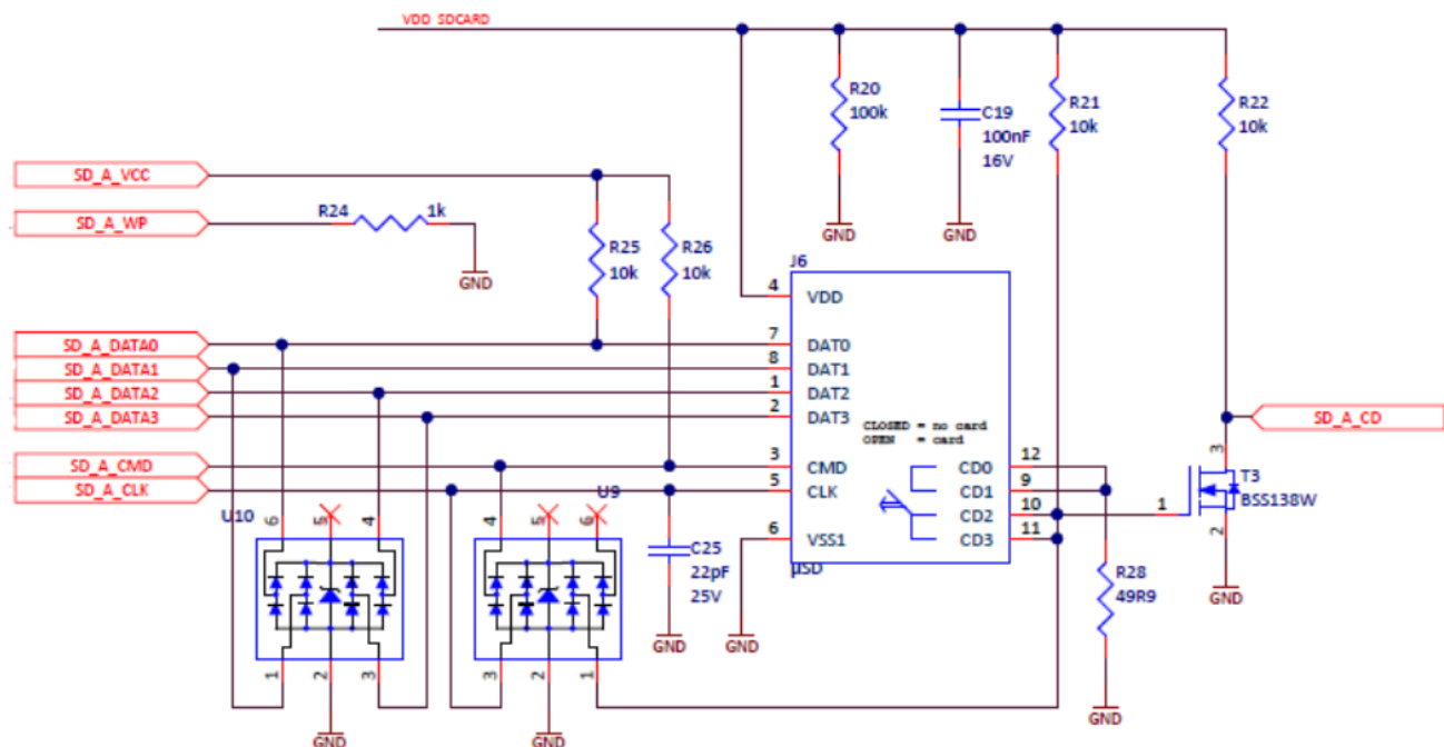
Figure 6: SD Card connector example connection
