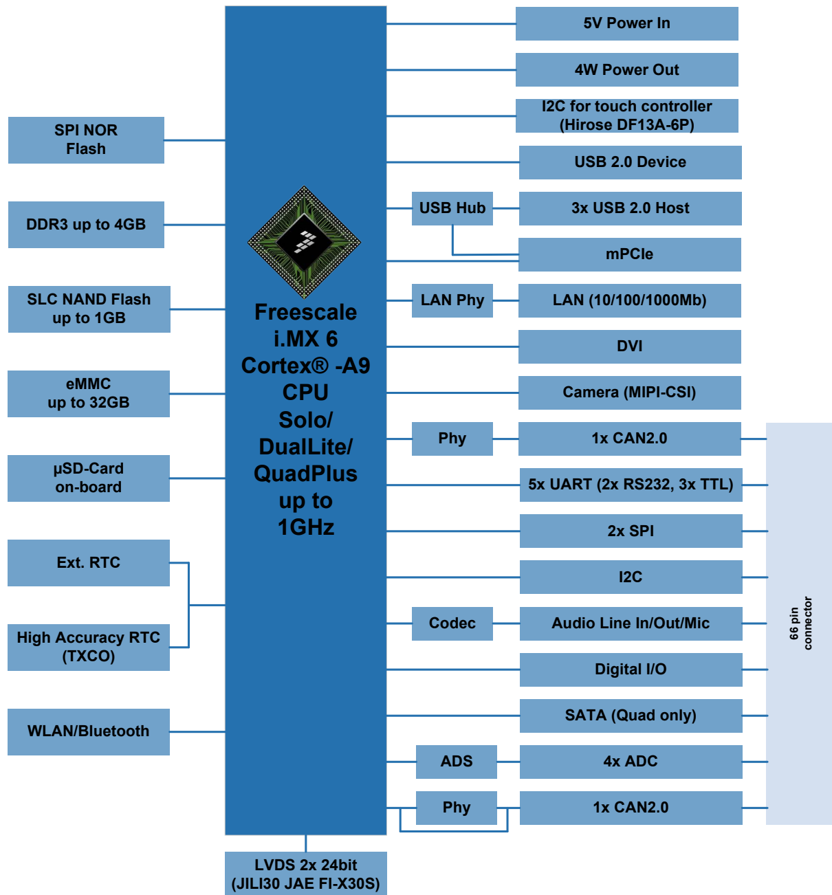
Figure 1: Block Diagram
